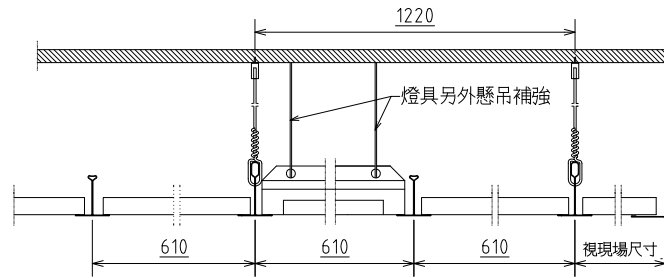
C-C SECTION
