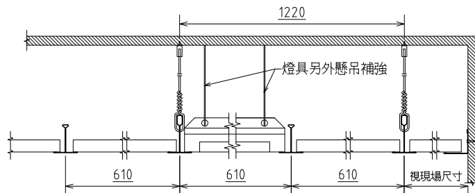
C-C SECTION
