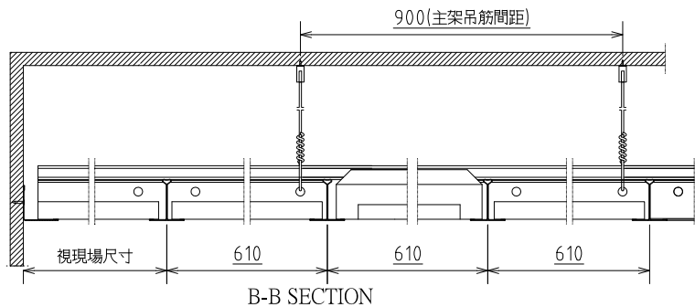
B-B SECTION
