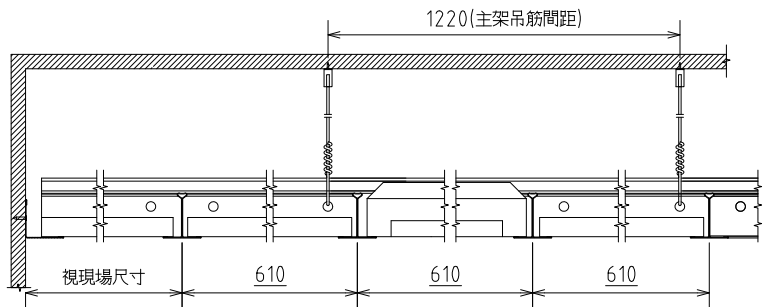
B-B SECTION
