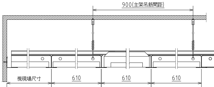
B-B SECTION
