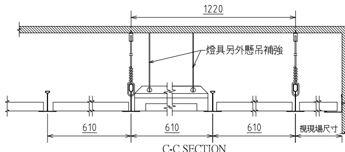
C-C SECTION
