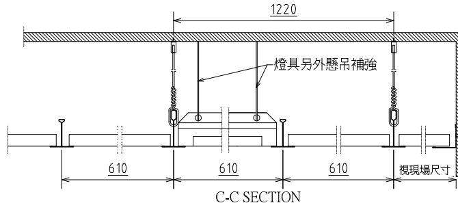
C-C SECTION
