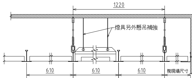
C-C SECTION
