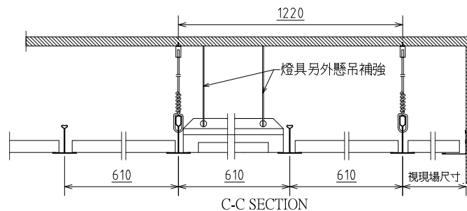
C-C SECTION
