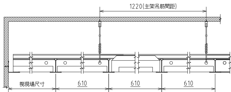
B-B SECTION
